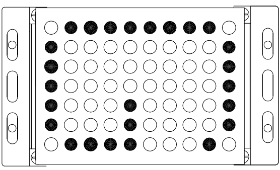
VERTICAL FLOOR DISPLAY SHOWING FLOOR LEVEL WITHOUT CALL BRACKET POSITION @ "B-B" 2 CHARACTER DISPLAY SIZE = 73.4mm
