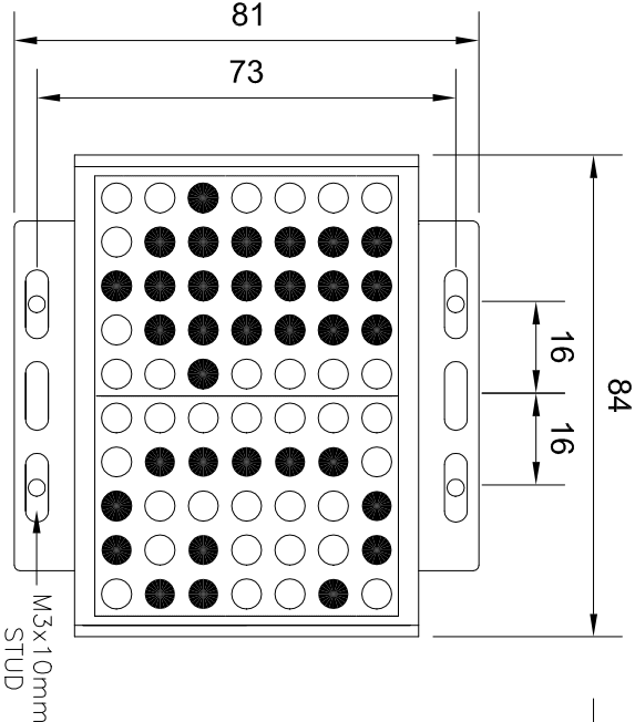
HORIZONTAL CAR DISPLAY SCROLLING CAR DIRECTION & FLOOR LEVEL
