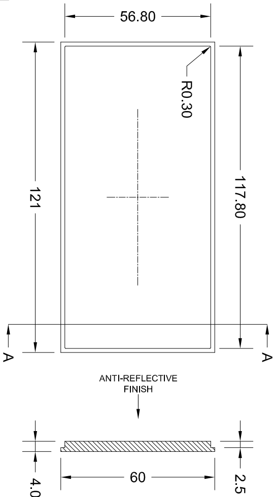
IND50*G LENS DETAIL 0.3mm INTERNAL RADIUS ON ALL CORNERS MATERIAL Smoke Grey Transparent (Dark Neutral) Cats Acrylic with Anti-Reflective Finish.
