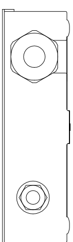
RHS VIEW Shown without lid
