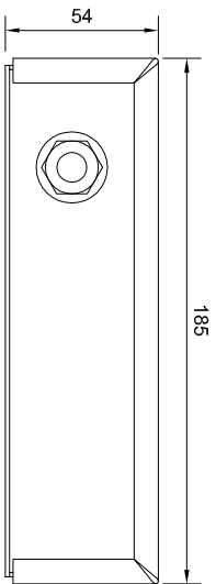
LHS VIEW Shown with lid
