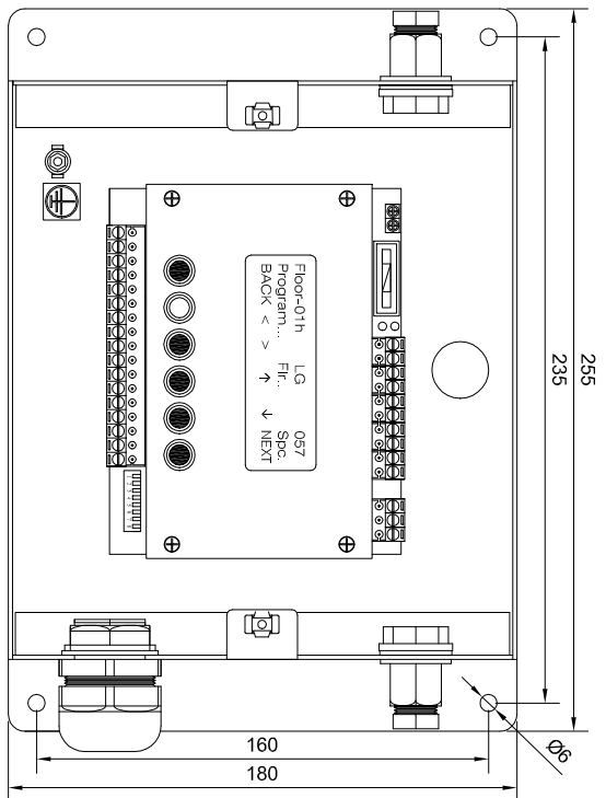
PLAN VIEW Shown without lid
